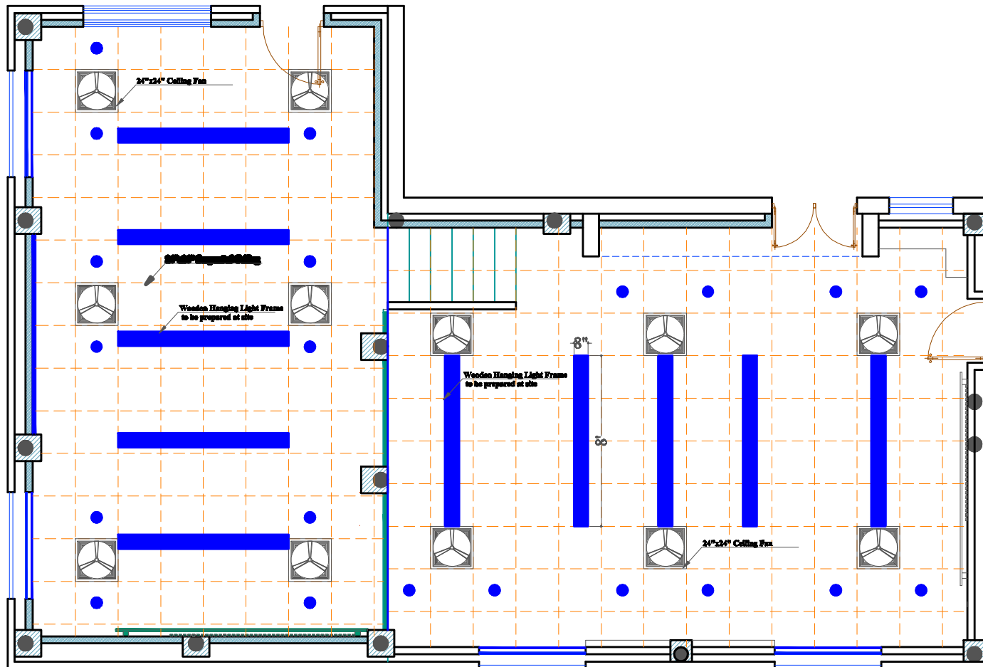
CEILING PLAN OF CAFETERIA AT UNHCR SUB OFFICE QUETTA
