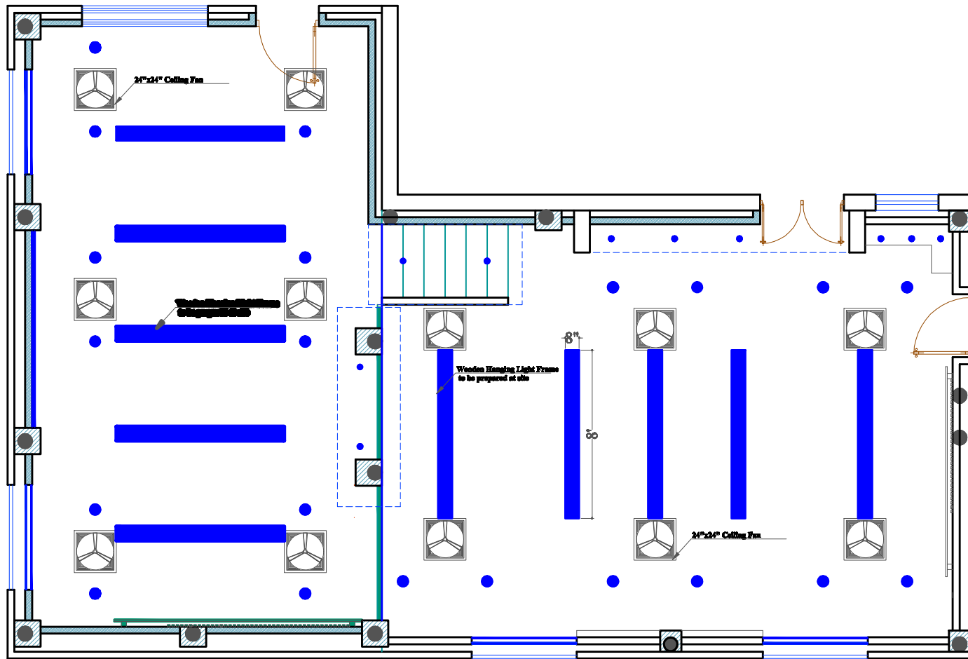
LIGHTING LAYOUT PLAN OF CAFETERIA AT UNHCR SUB OFFICE QUETTA
