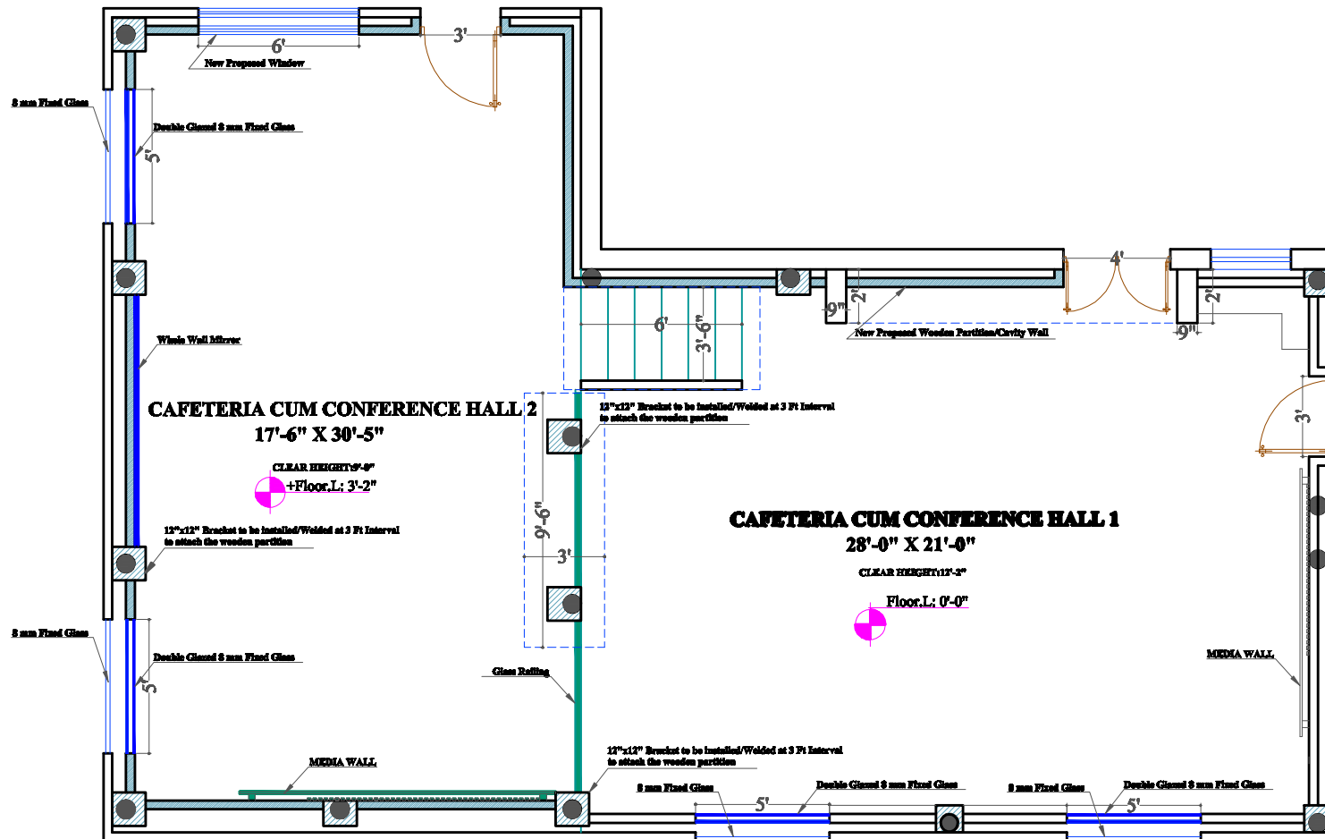
PROPOSED PLAN OF CAFETERIA AT UNHCR SUB OFFICE QUETTA
