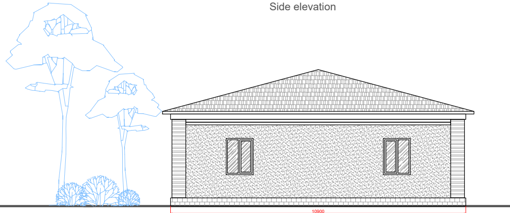
Rear elevation
