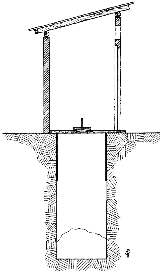
Figure 3 - Diagram of a pit latrine with a slab fitted with a lid
