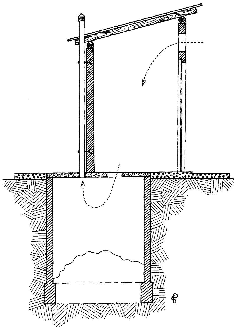
Figure 2 - Diagram of a ventilated improved pit latrine
